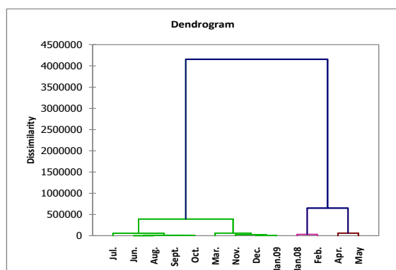
Figure 2: Dendrogram showing similarity of Zooplankton density at station 1.
